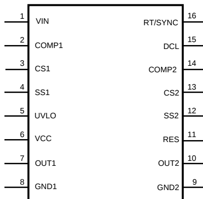
Pin Functions
